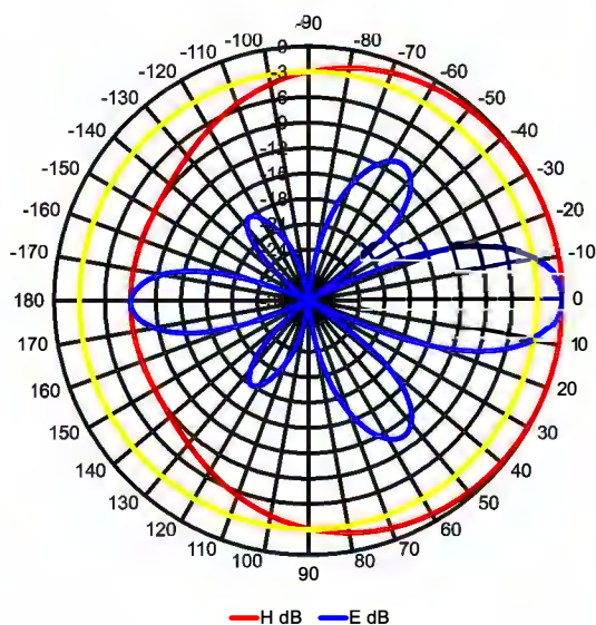
RADIATION PATTERN
