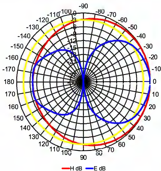
RADIATION PATTERN VHF
