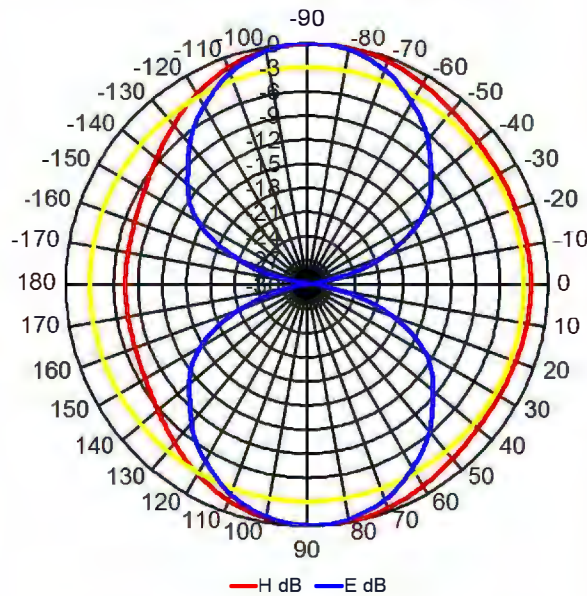
RADIATION PATTERN UHF
