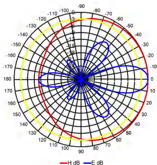
RADIATION PATTERN
